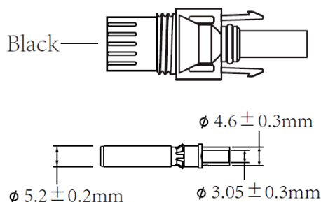
Pic 5.1 DC+ male connector
