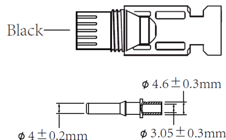
Pic 5.2 DC- female connector
